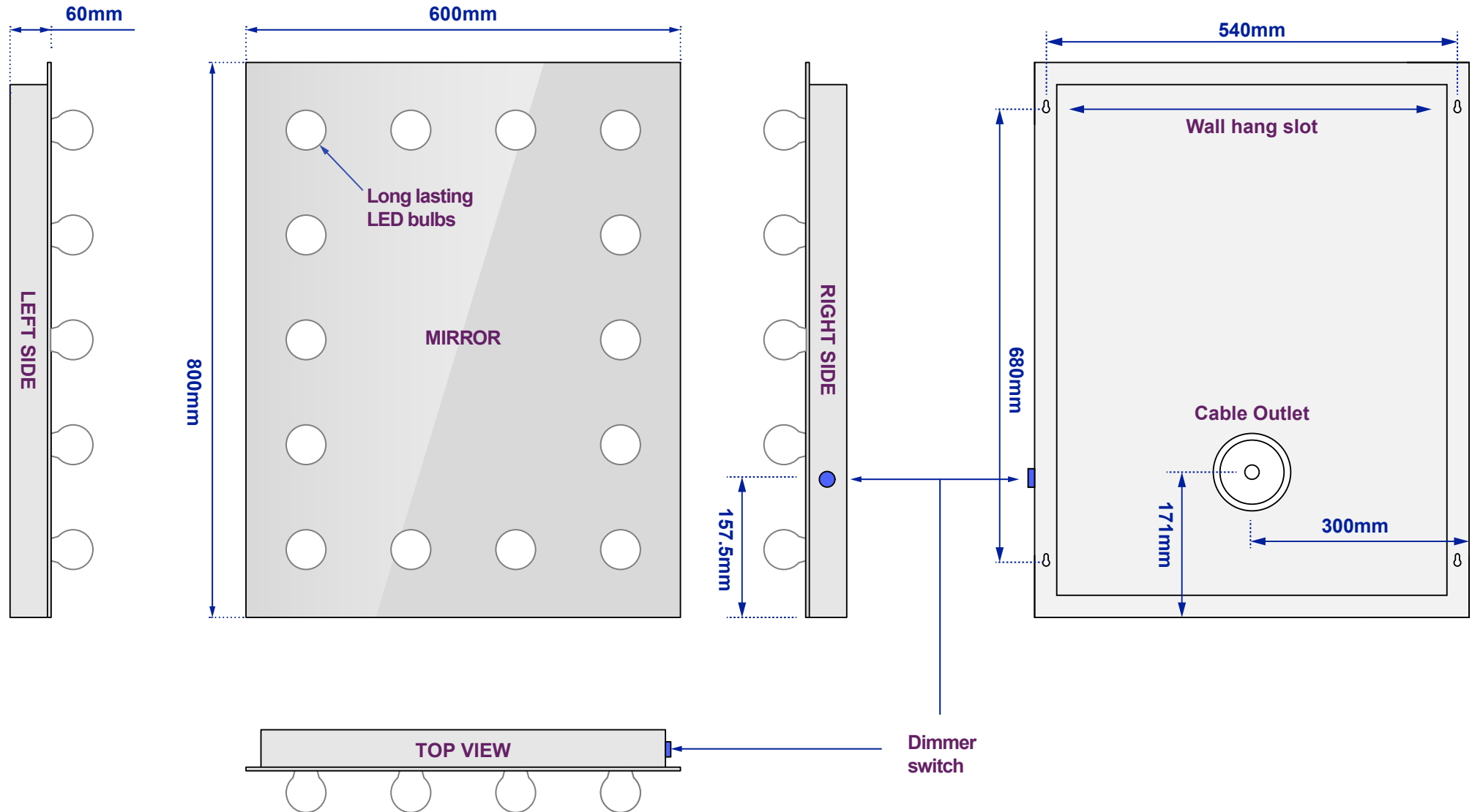
Views of completed assembly - with bulbs in place
