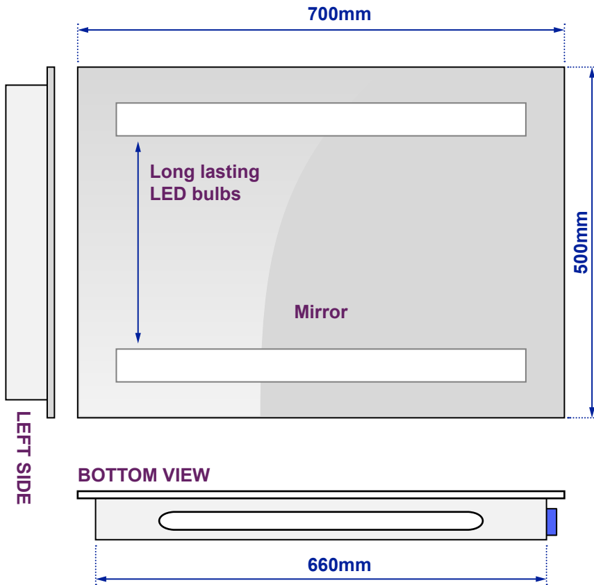
Views of complete assembly - With Mirror
